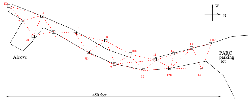
Fig. 7. Sensor network layout. The solid line plots the service road. The sensor nodes are marked with small squares. Labels with a “D” are DOA sensors. The dashed lines picture the connectivity between nodes.
